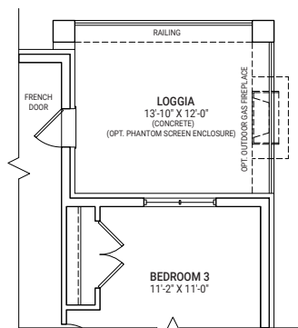
PARTIAL GROUND FLOOR PLAN W/ OPT. LOGGIA
