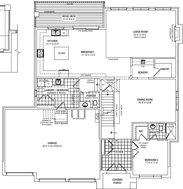
GROUND FLOOR PLAN ELEVATION D
